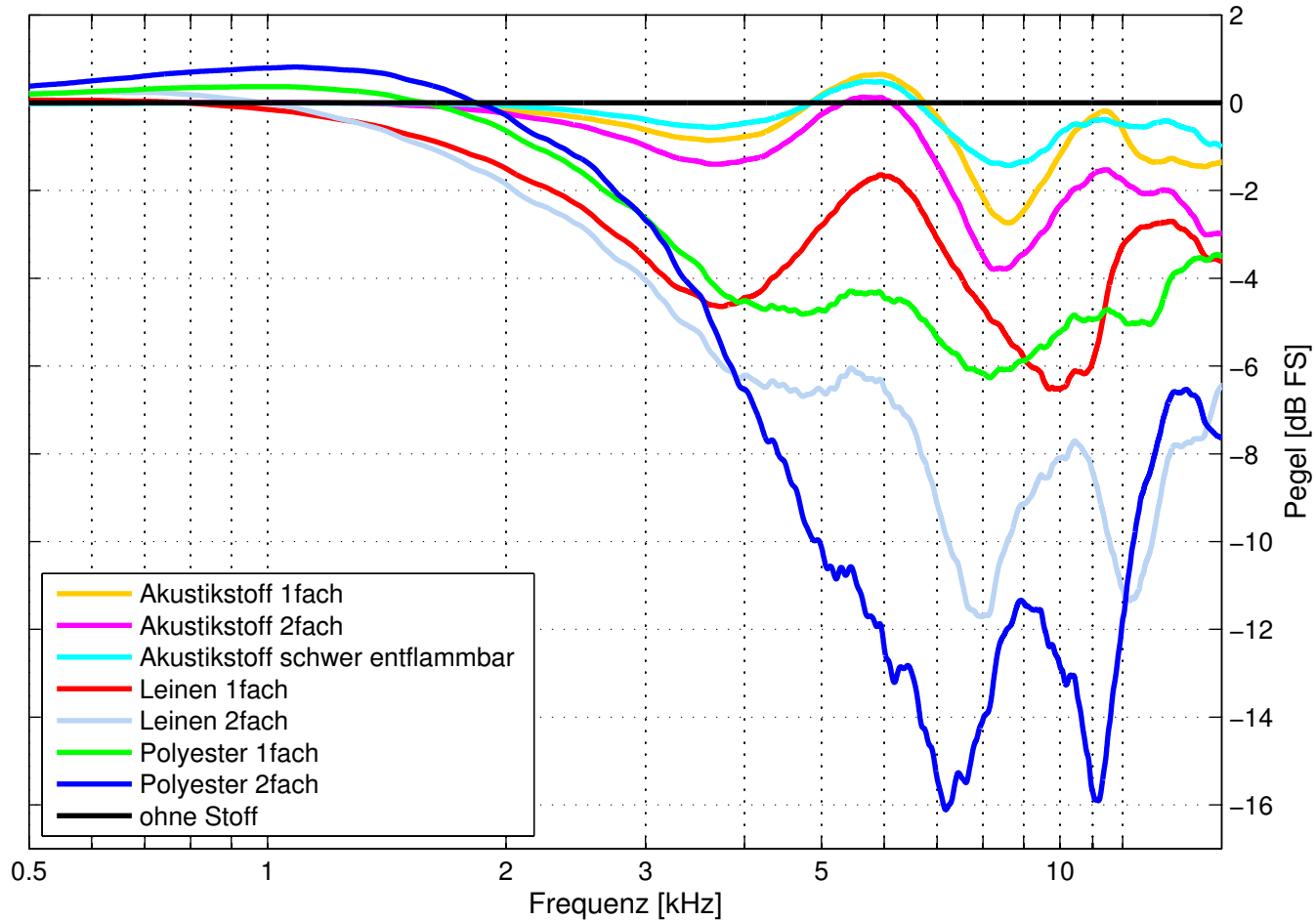
Sweep Signal (100 – 20k Hz), Fostex 6301B → B&K 40AF
